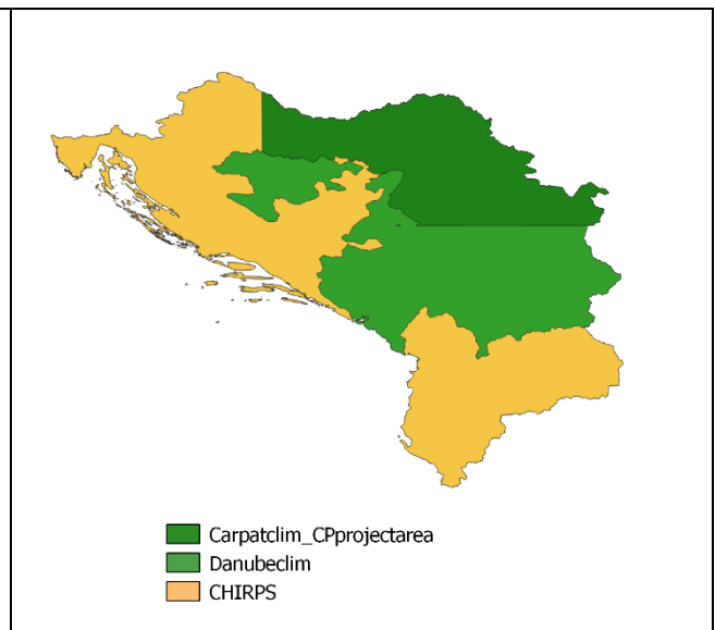
Figure 3: Observational Data used for Bias Correction of Precipitation; (Illustrated by BOKU-Met, Datasource: Diva-gis, Carpatclim, Danubeclim, CHIRPS)
